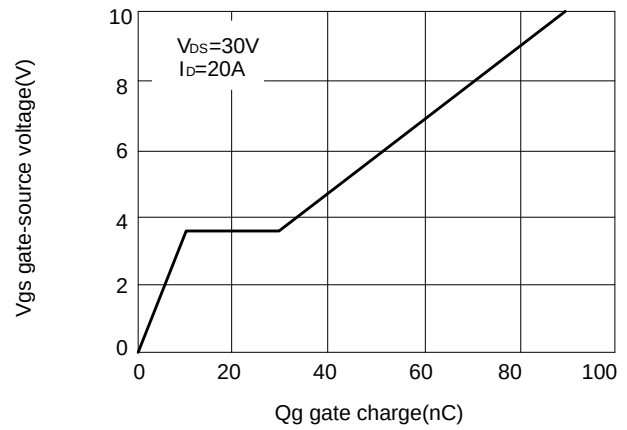
Figure 4: Gate charge
