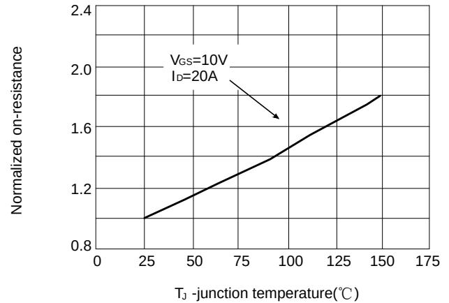
Figure 2: R_{DS(on)} -junction temperature
