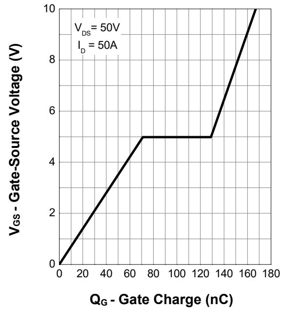
Gate Charge
