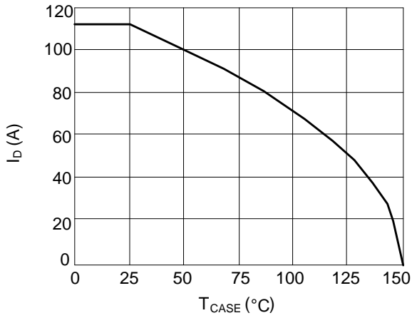
Figure 7: Current de-rating
