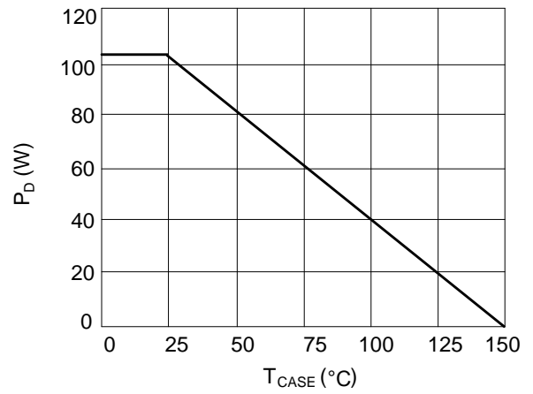
Figure 8: Power de-rating
