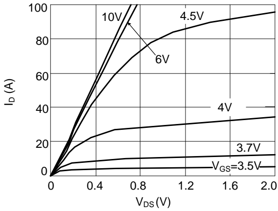
Figure 1: Saturation characteristics
