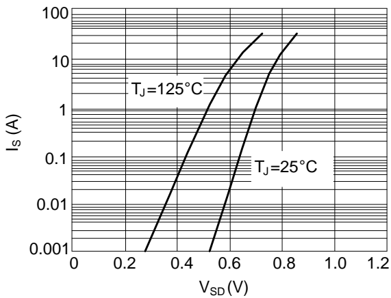
Figure 5: Body-diode characteristics
