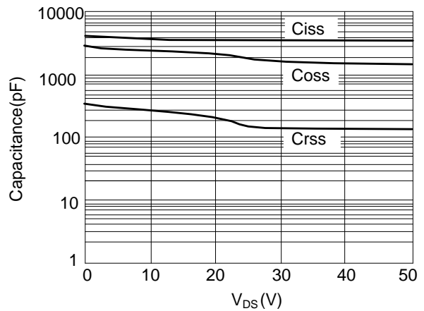
Figure 6: Capacitance characteristics
