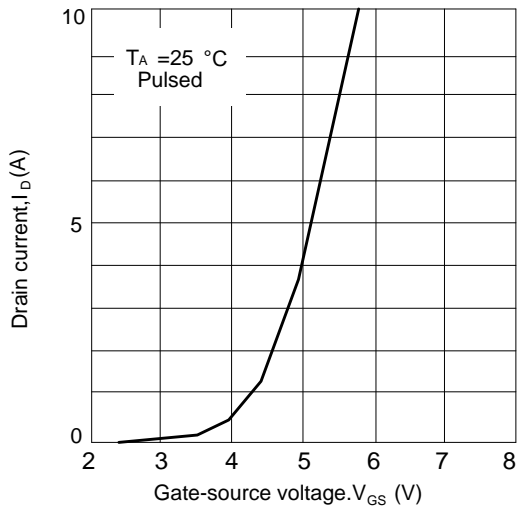
Figure 9: Drain current vs. case-source voltage
