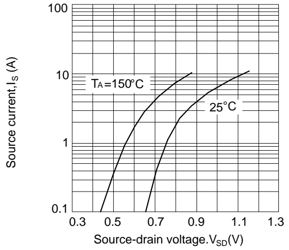
Figure 2: Source current vs. source-drain voltage
